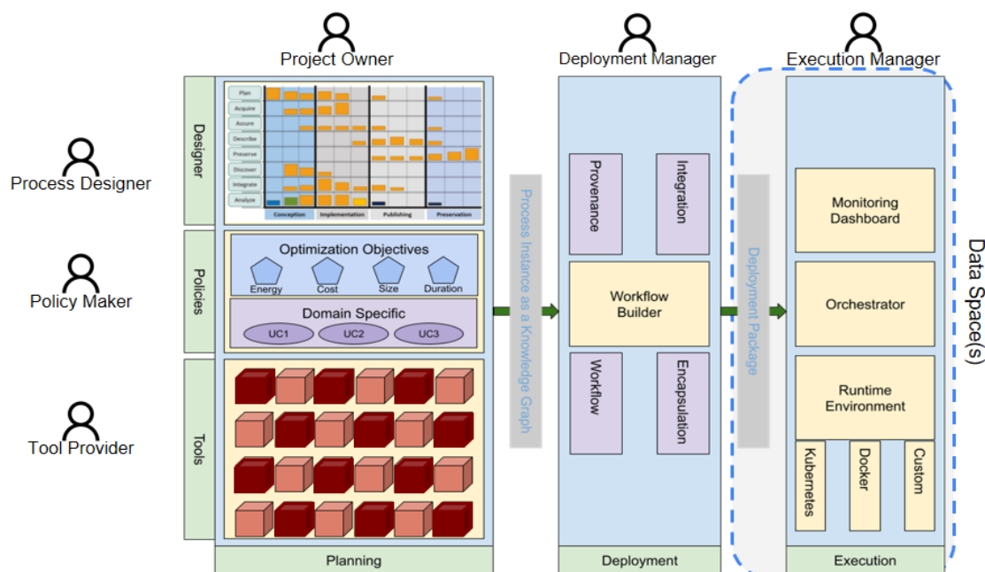
Figure 1 "DataBri-X Architecture"
