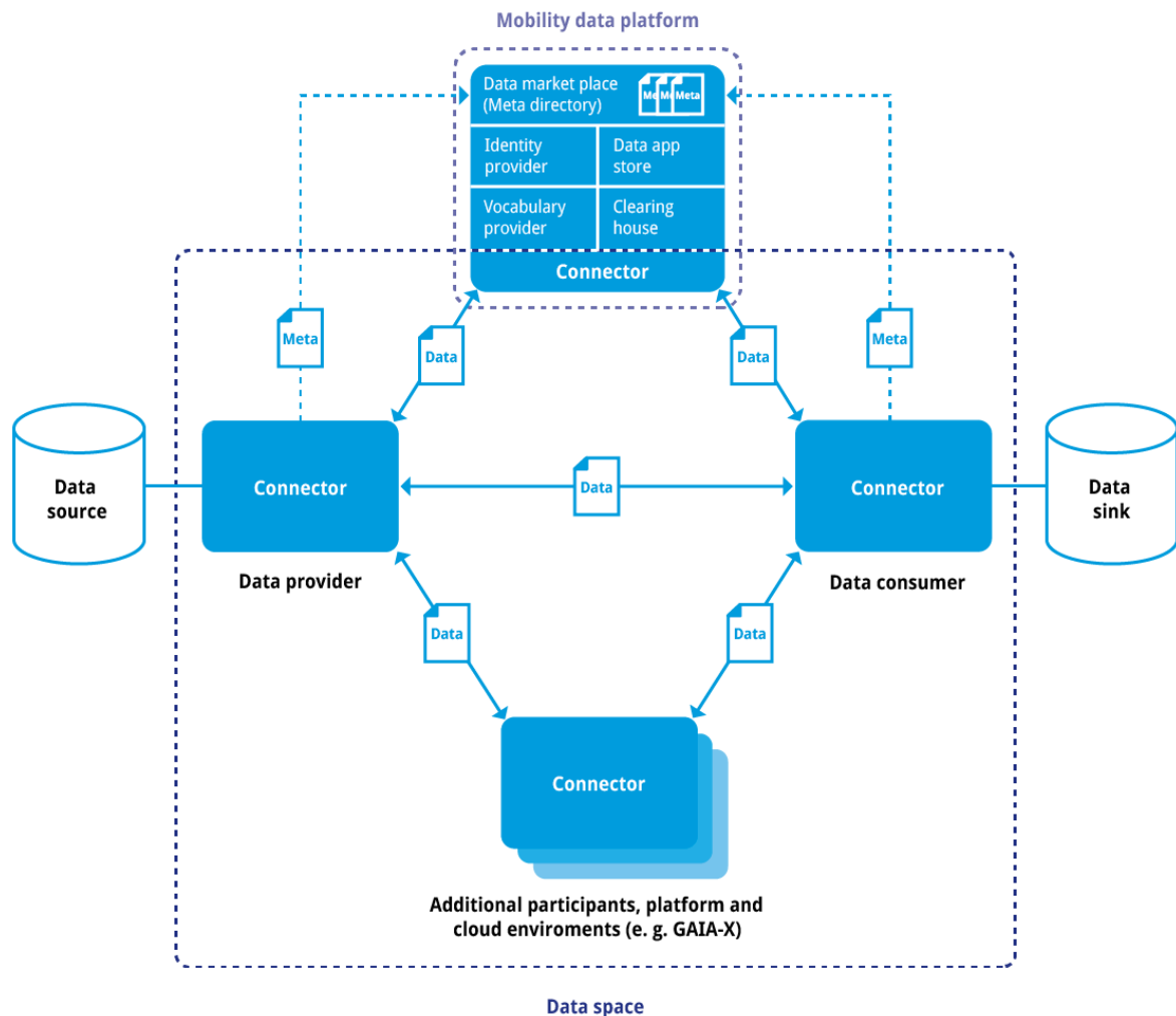
Figure 2: secure data space
