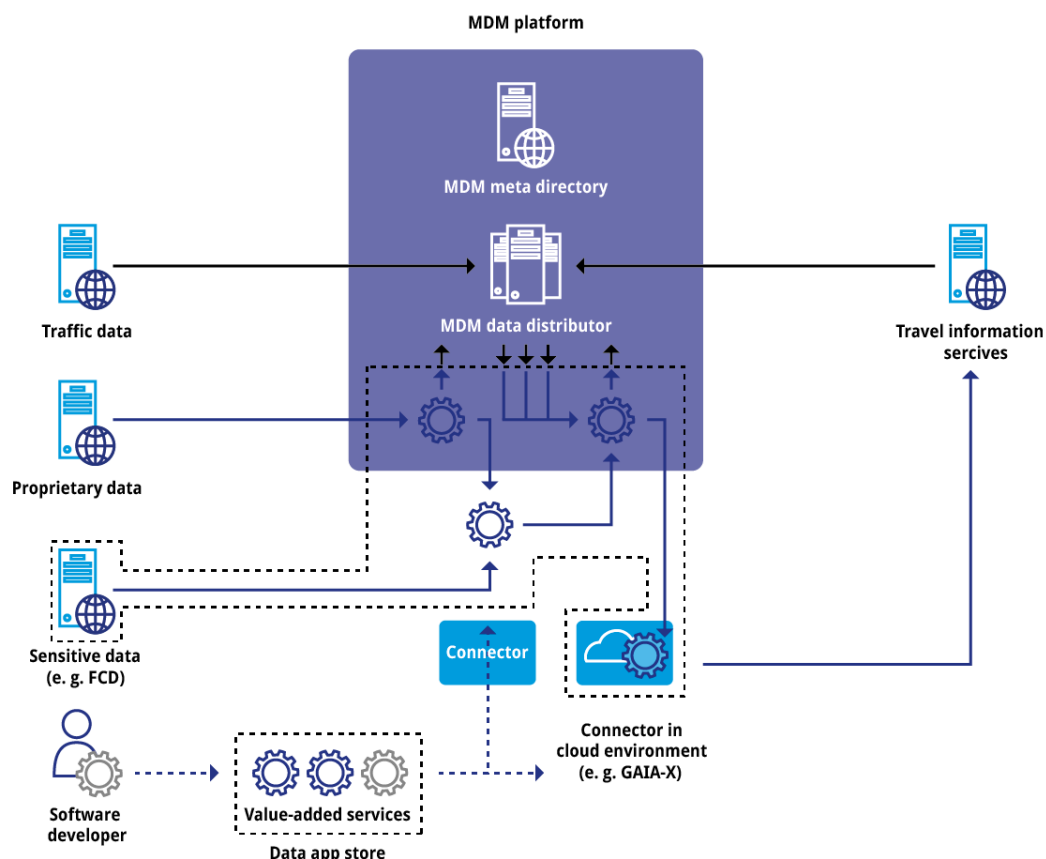
Figure 3: The MDM, extended by an IDS connector, as part of the Mobility Data Space.
